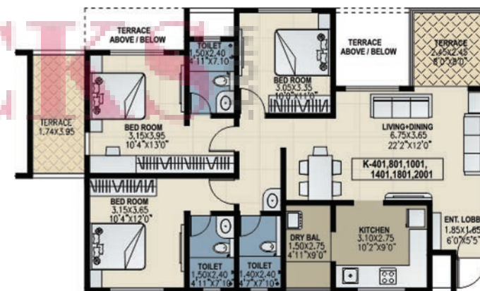
BUILDING K 3 BHK - EVEN FLOOR FLAT CARPET - 94.32 sq m TERRACE CARPET - 12.89 sq m TOTAL CARPET - 107.21 sq m
