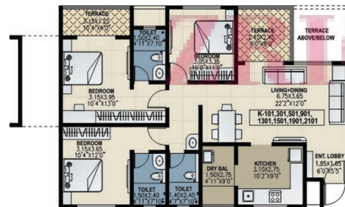
BUILDING K 3 BHK - ODD FLOOR FLAT CARPET - 94.47 sq m TERRACE CARPET - 9.94 sq m TOTAL CARPET - 104.41 sq m
